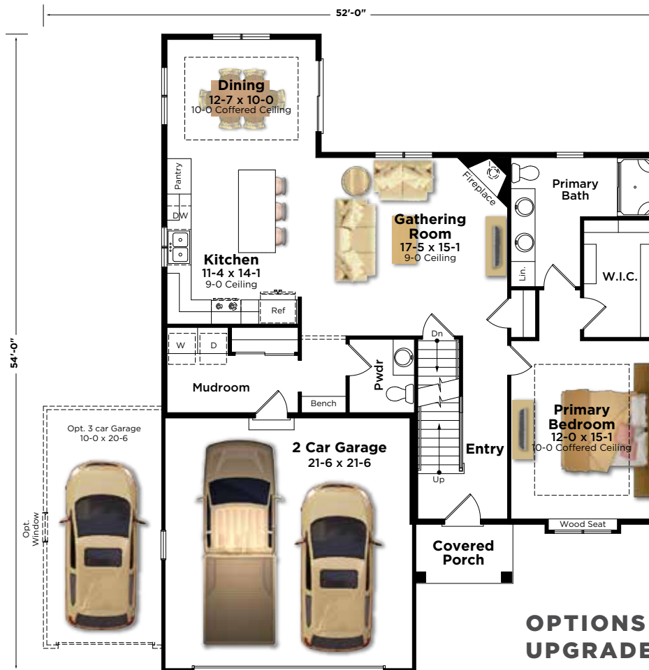
First Floor 1,269 Square Feet
